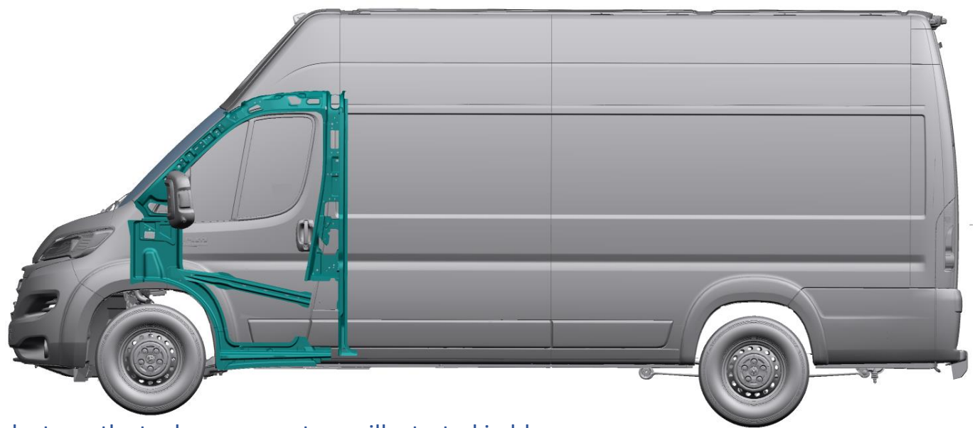
High strength steel components are illustrated in blue-green.
